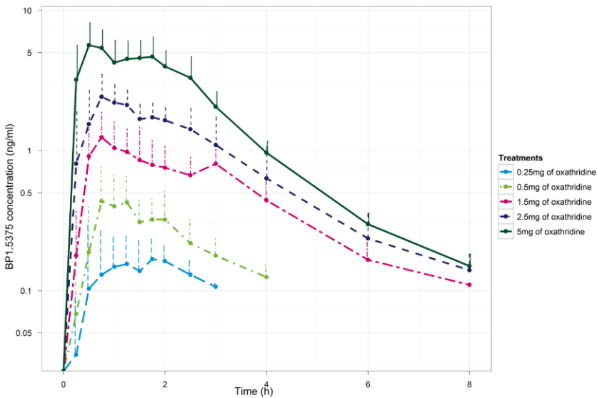
Figure 1 Pharmacokinetics of oxathridine
